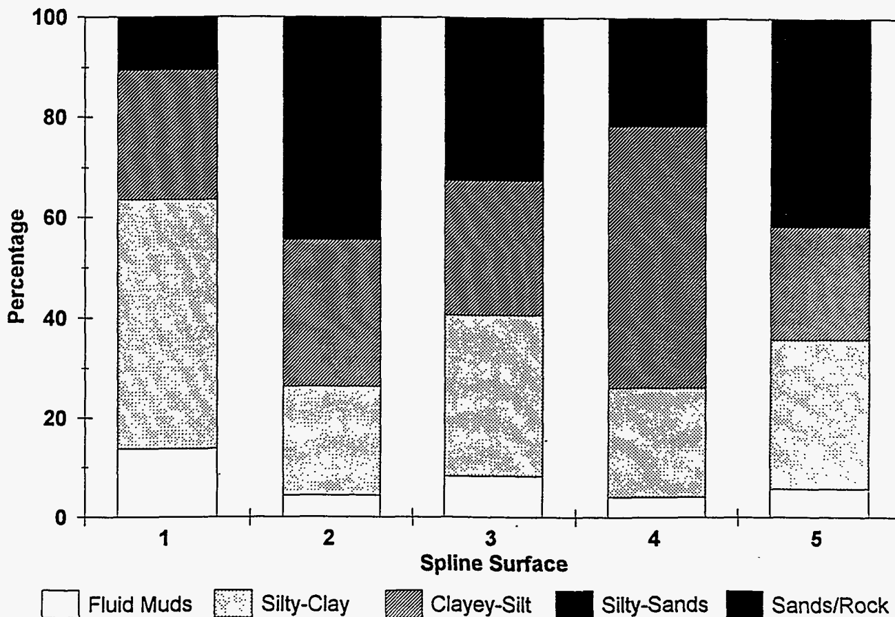
Figure 1: Surface sediment types for each spline scenario
